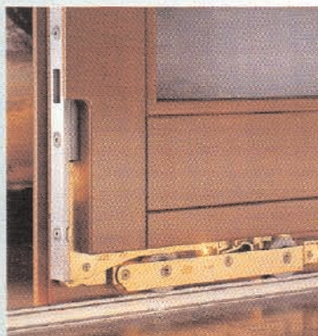
AGB AS-250 Lift-slide (550lbs. capacity)
