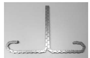
double zipper SST chain
