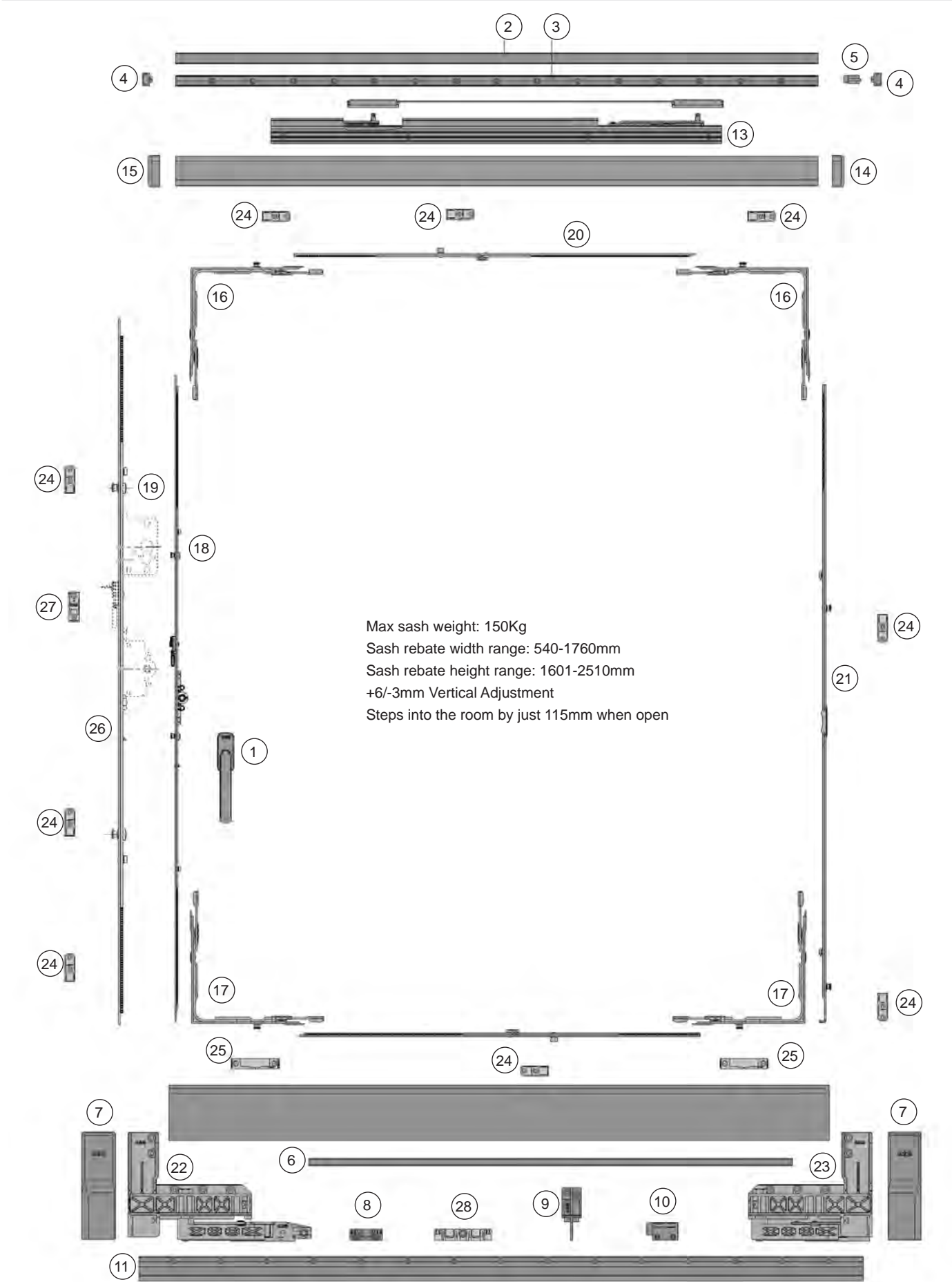
AGB Galileo CM Tilt/Slide Patio Hardware for Scheme 'A' Door
